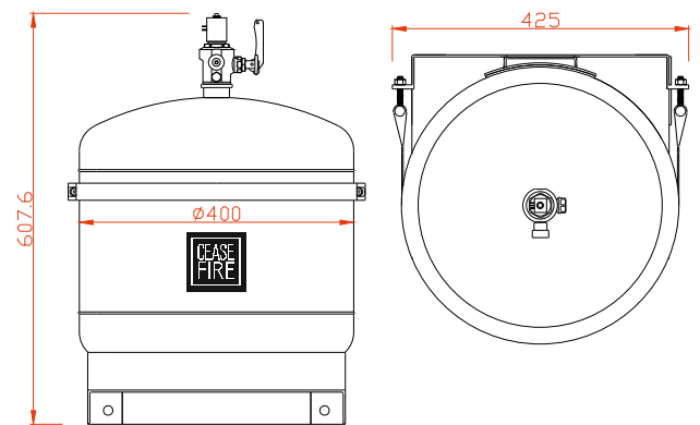
Ceasefire ULtraX KSS 44 Ltr SS Container with Mechanical Valve, Pressure Gauge, SS Dip Tube, Agent 30 Ltr, Bracket & Marking Label, Product code CF-001281
