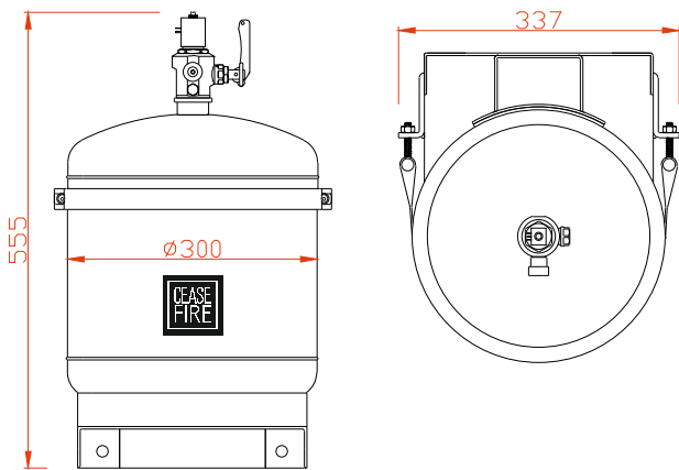
Ceasefire ULtraX KSS 22 Ltr SS Container with Mechanical Valve, Pressure Gauge, SS Dip Tube, Agent 16.5 Ltr, Bracket & Marking Label, Product code CF-001278
