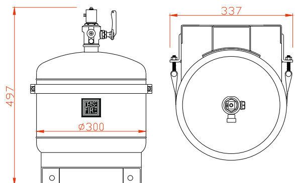
Ceasefire UltraX KSS 18 Ltr SS Container with Mechanical Valve, Pressure Gauge, SS Dip Tube, Agent 12 Ltr, Bracket & Marking Label, Product code CF-000669AD
