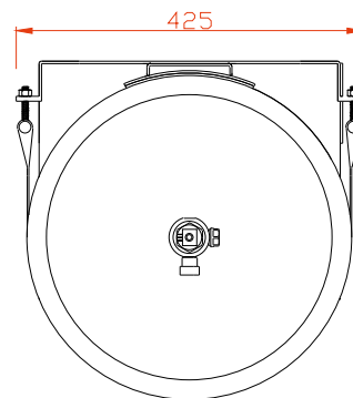
Ceasefire ULtraX KSS 64 Ltr SS Container with Mechanical Valve, Pressure Gauge, SS Dip Tube, Agent 45 Ltr, Bracket & Marking Label, Product code CF-001282
