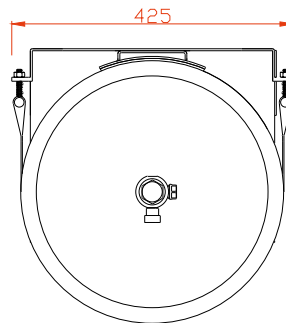
Ceasefire UltraX KSS 64 Ltr SS Container with Mechanical Valve, Pressure Gauge, SS Dip Tube, Agent 45 Ltr, Bracket & Marking Label, Product code CF-001573
