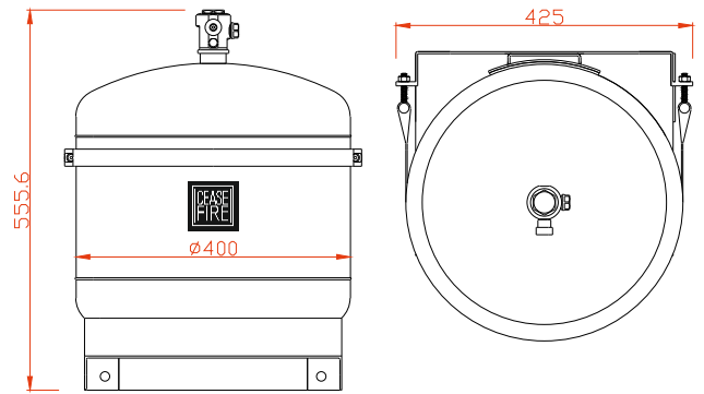
Ceasefire UltraX KSS 44 Ltr SS Container with Mechanical Valve, Pressure Gauge, SS Dip Tube, Agent 30 Ltr, Bracket & Marking Label, Product code CF-001572
