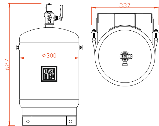
Ceasefire ULtraX KSS 27 Ltr SS Container with Mechanical Valve, Pressure Gauge, SS Dip Tube, Agent 20 Ltr, Bracket & Marking Label, Product code CF-000669BD
