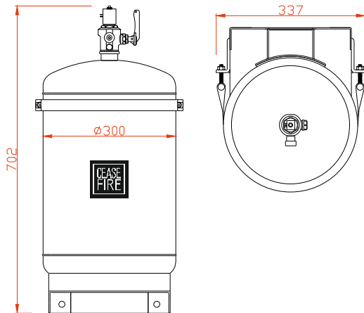
Ceasefire ULtraX KSS 32 Ltr SS Container with Mechanical Valve, Pressure Gauge, SS Dip Tube, Agent 24 Ltr, Bracket & Marking Label, Product code CF-001280
