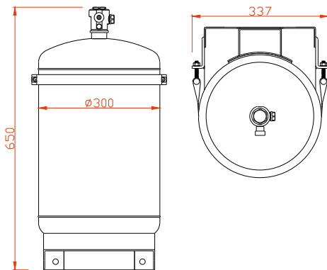
Ceasefire UltraX KSS 32 Ltr SS Container with Mechanical Valve, Pressure Gauge, SS Dip Tube, Agent 24 Ltr, Bracket & Marking Label, Product code CF-001571
