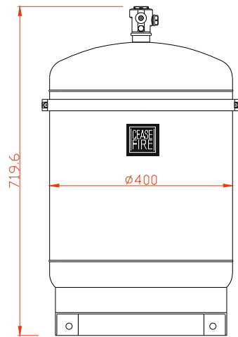
Ceasefire UltraX KSS 32 Ltr SS Container with Mechanical Valve, Pressure Gauge, SS Dip Tube, Agent 24 Ltr, Bracket & Marking Label, Product code CF-001571
